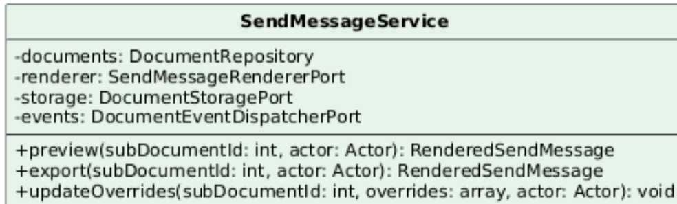
Figura 30: Classe — SendMessageService
