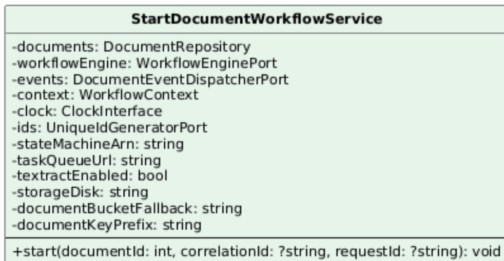
Figura 21: Classe — StartDocumentWorkflowService
