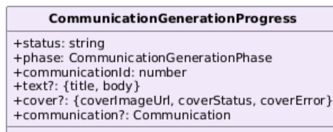
Figura 95: Tipo — CommunicationGenerationProgress
